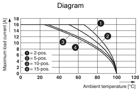
Derating curve for ST 2,5-TWIN-MT/1P, ST 2,5-TWIN-TG/1P and for all plug versions SP...
