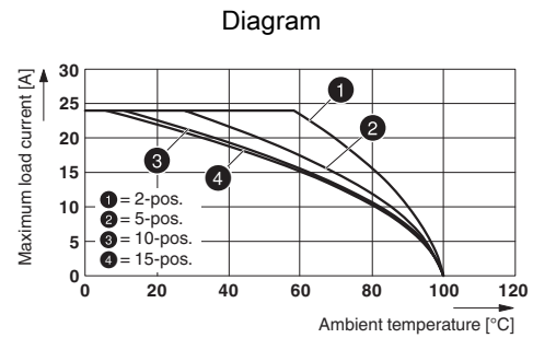
Derating curve for ST 2,5-QUATTRO/2P, ST 2,5-QUATTRO/4P and for all plug versions SP...
