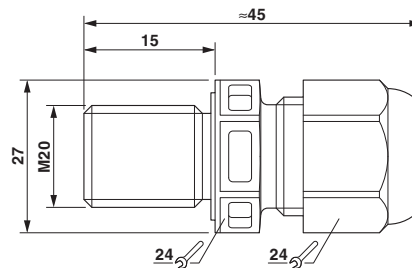
Dimensional drawing
