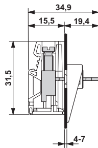
Dimensional drawing
