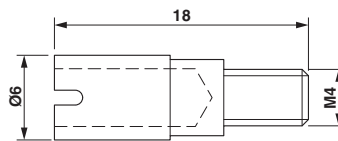
Dimensional drawing
