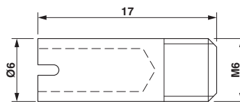
Dimensional drawing
