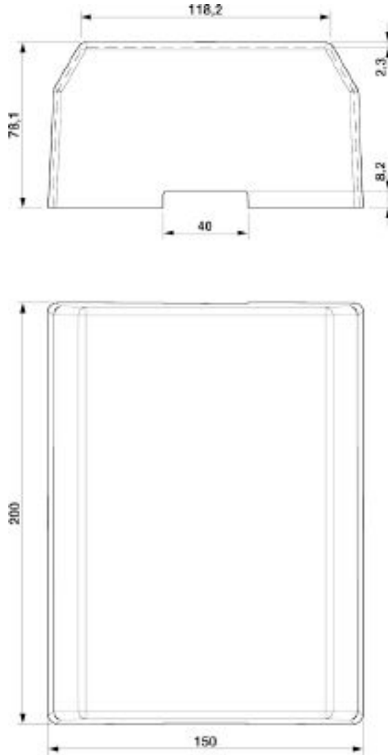
Dimensional drawing
