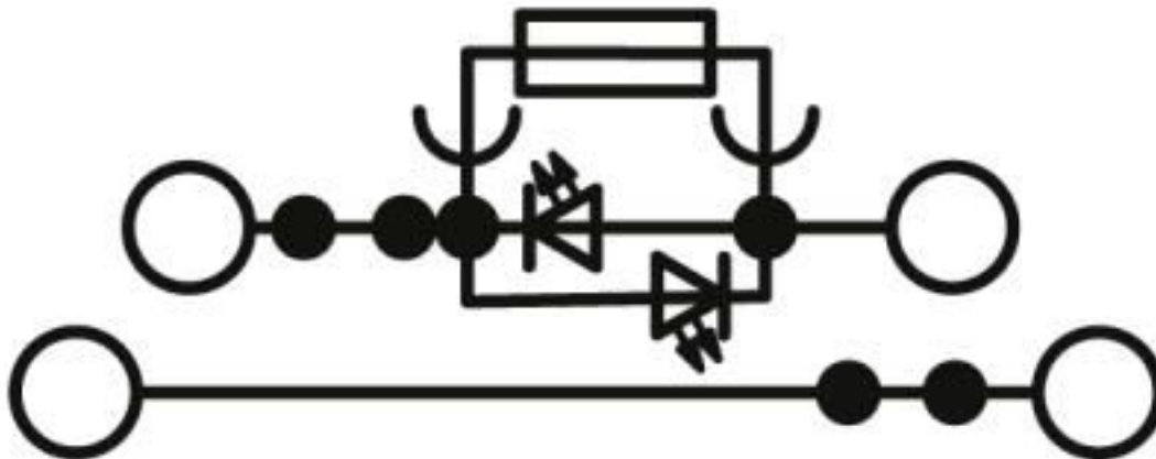
Circuit diagram
