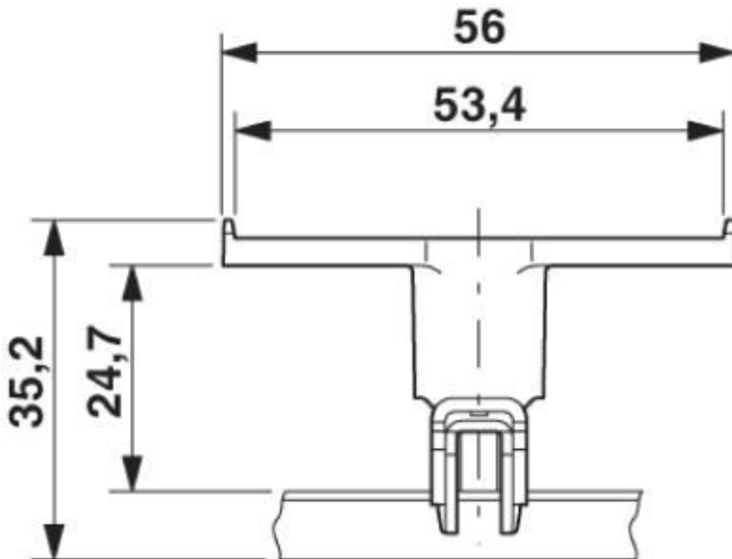
Dimensional drawing
