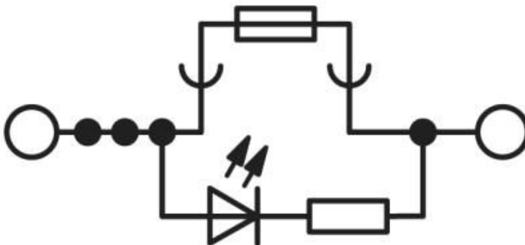
Circuit diagram
