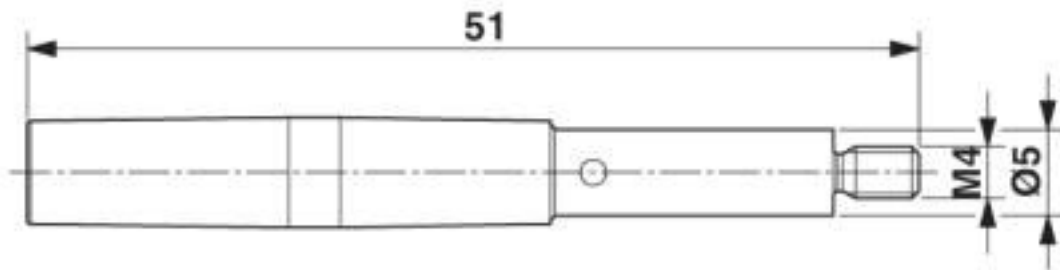
Dimensional drawing
