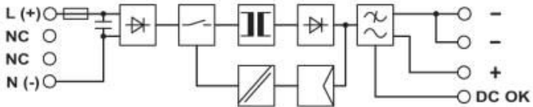
Block diagram
