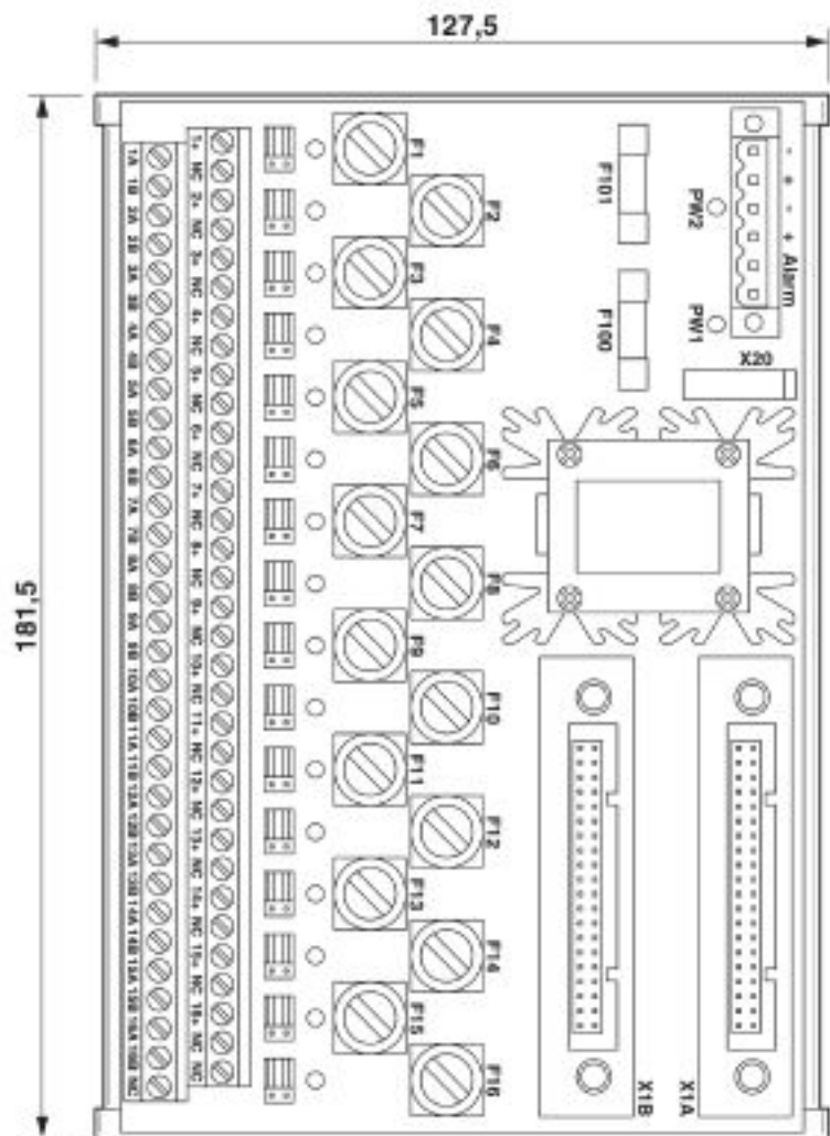
Dimensional drawing
