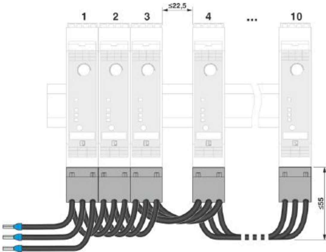
Application drawing
