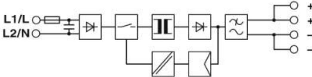
Block diagram
