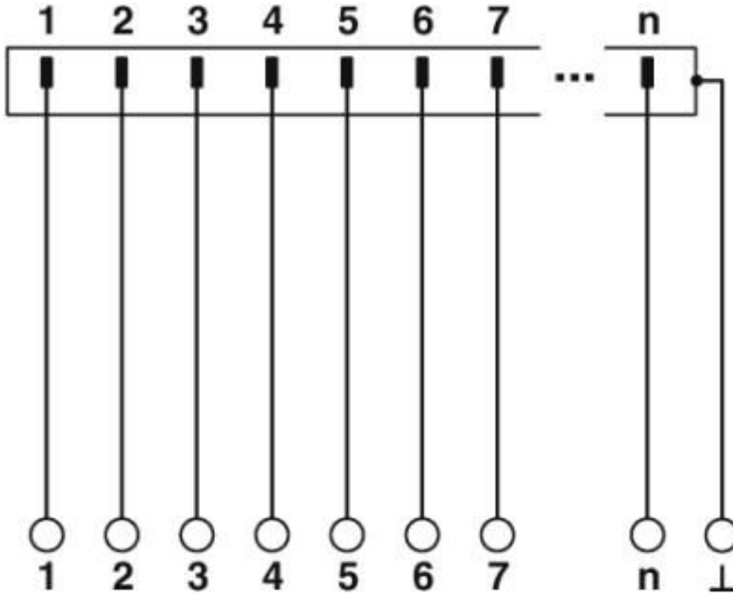
Circuit diagram
