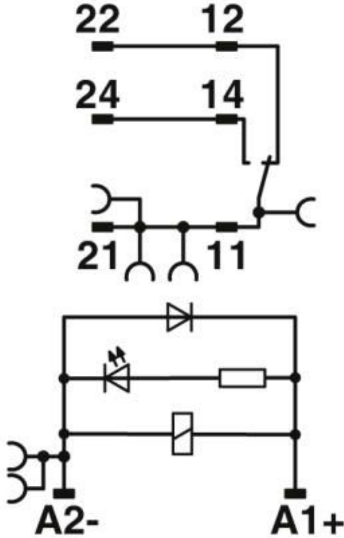
Circuit diagram
