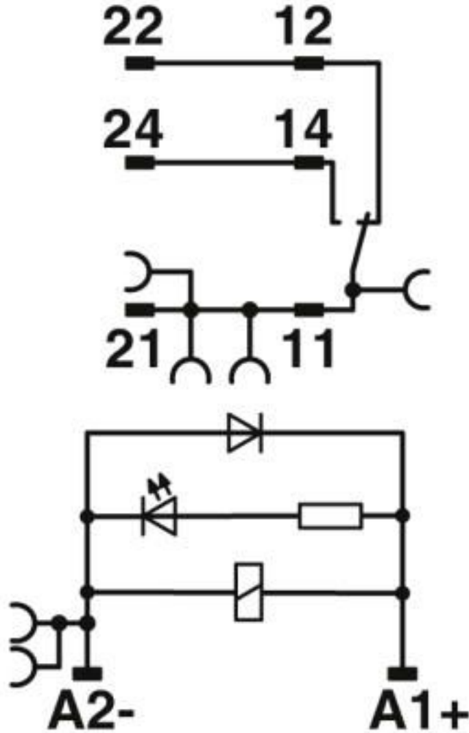
Circuit diagram
