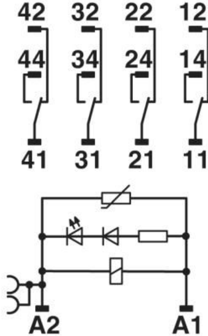
Circuit diagram
