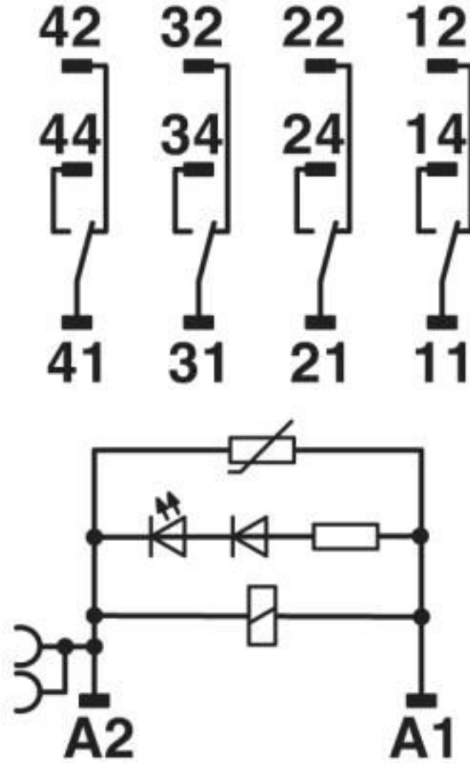
Circuit diagram
