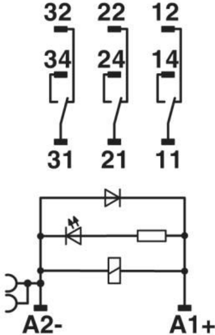
Circuit diagram
