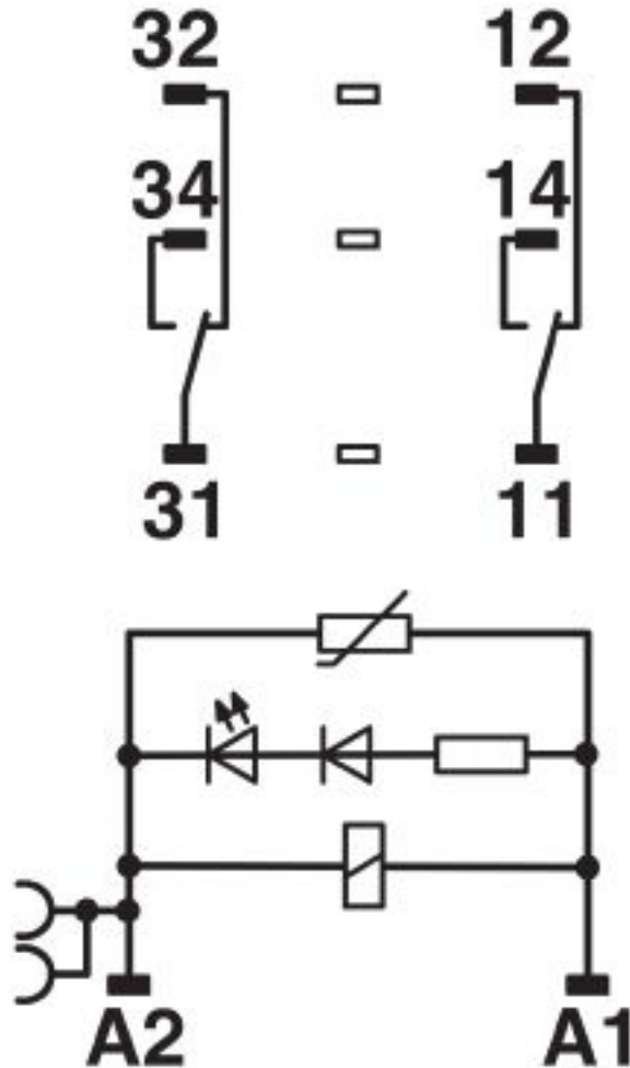
Circuit diagram
