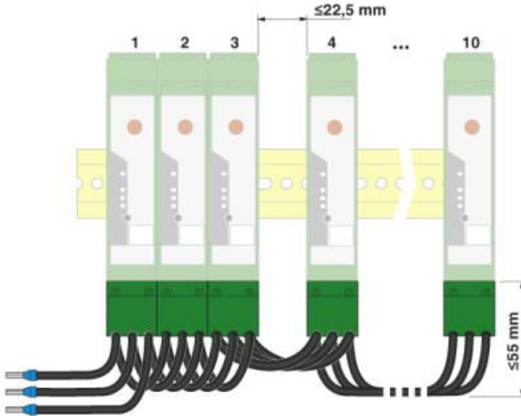
Application drawing
