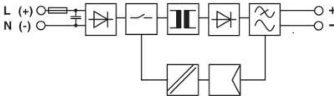
Block diagram
