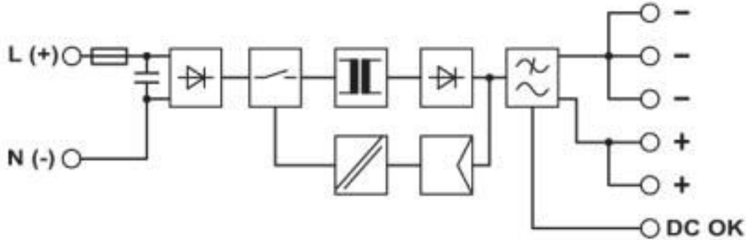
Block diagram
