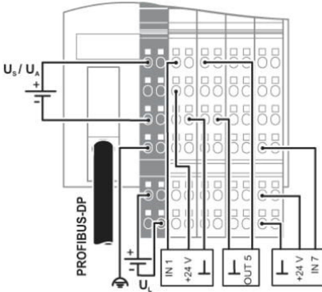
Connection diagram
