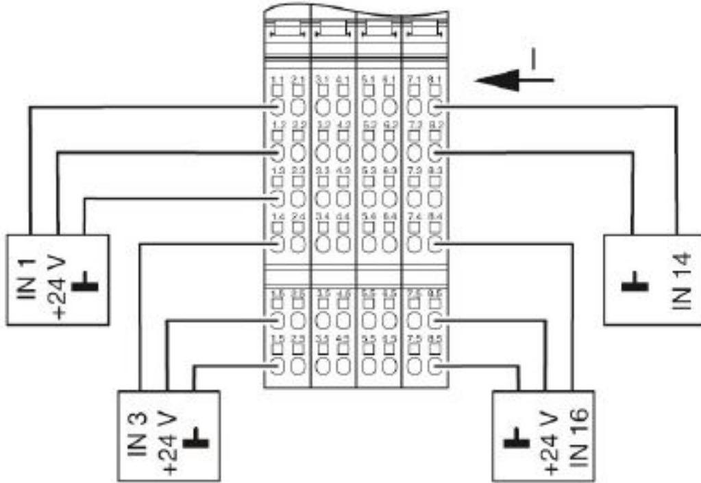
Connection diagram
