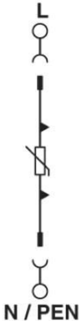
Circuit diagram
