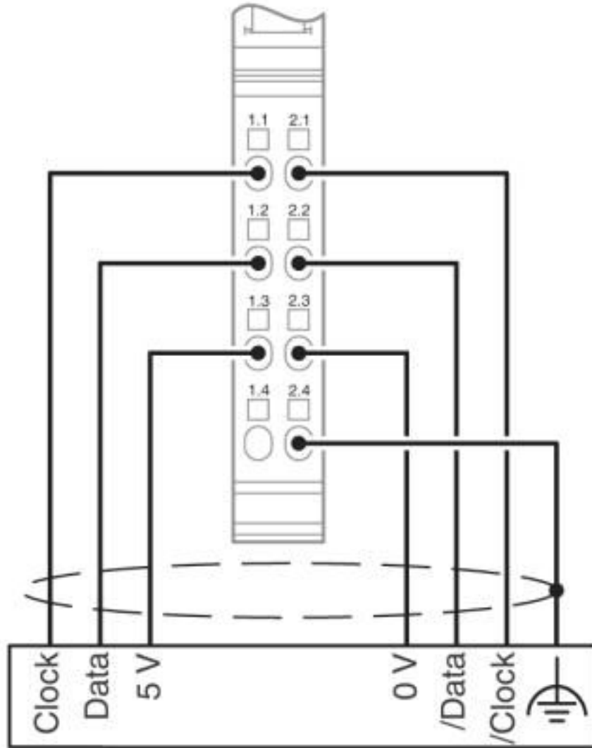
Connection diagram
