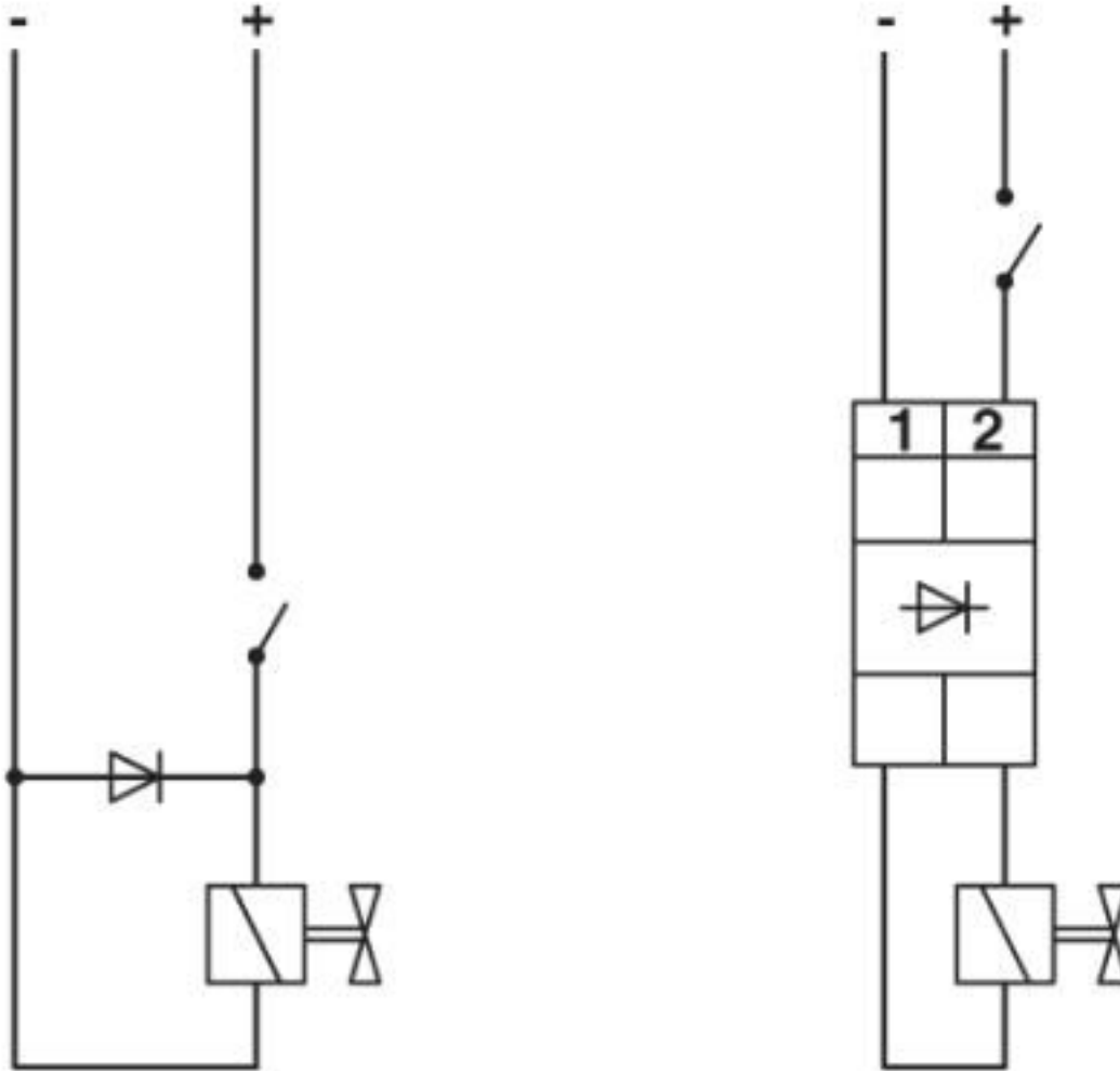
Circuit diagram
