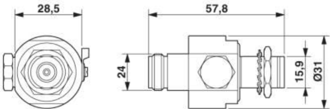
Dimensional drawing
