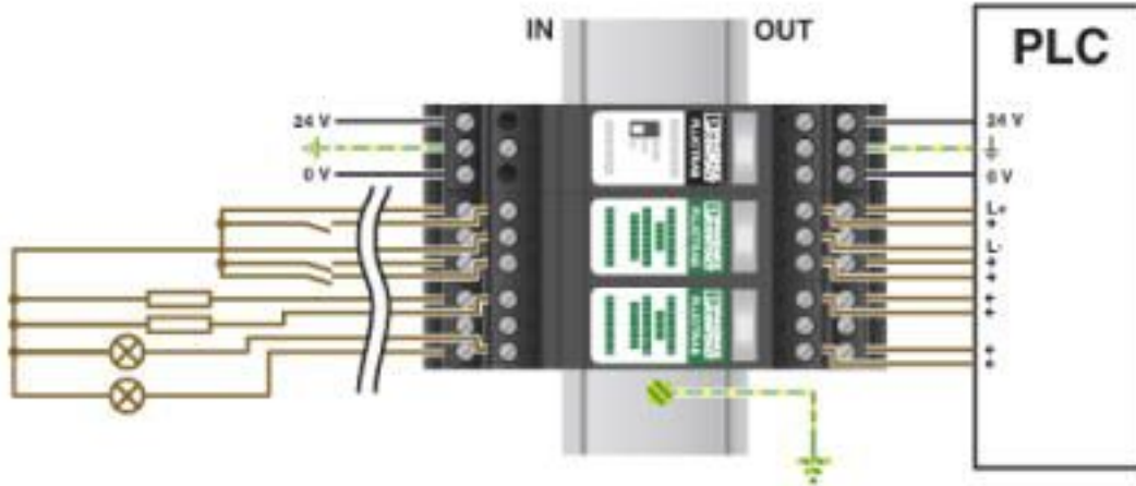
Application drawing
