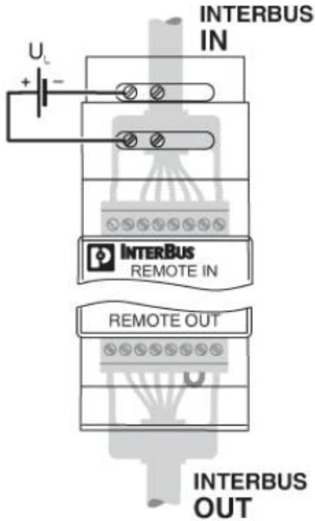
Connection diagram
