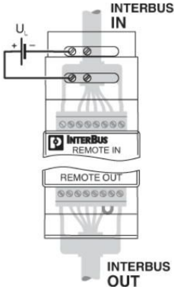
Connection diagram
