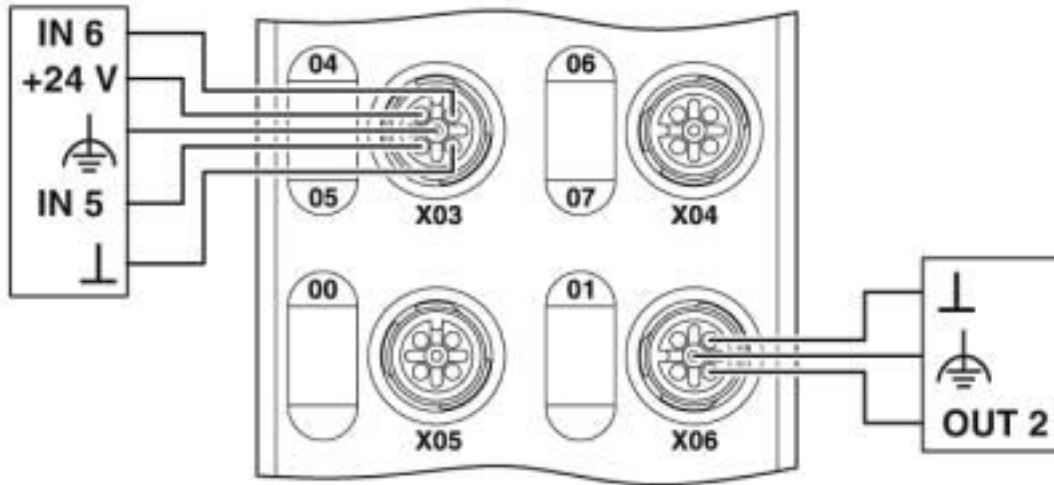
Connection diagram
