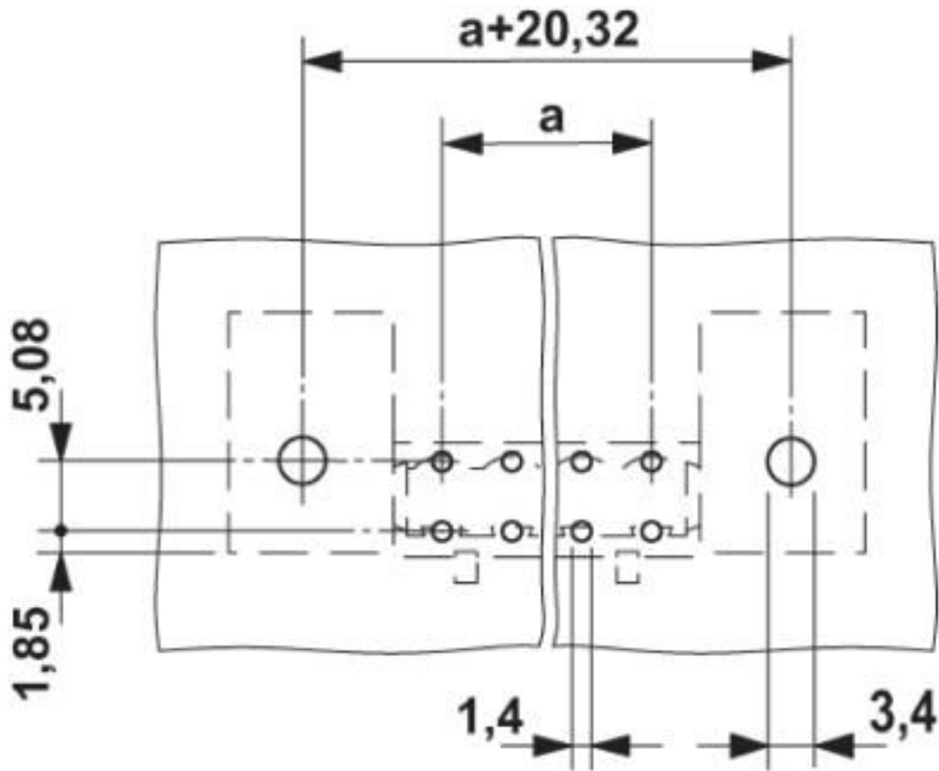
Drilling diagram
