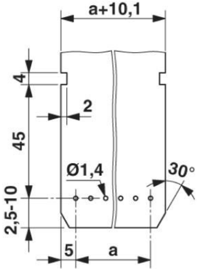
Drilling diagram
