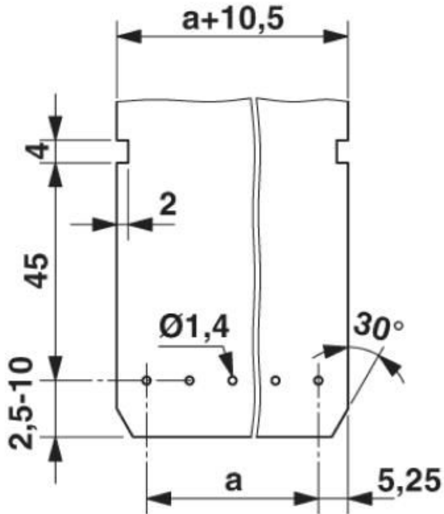
Drilling diagram
