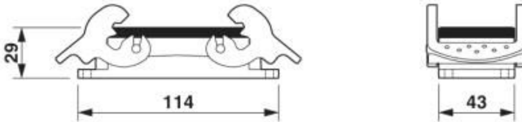
Dimensional drawing
