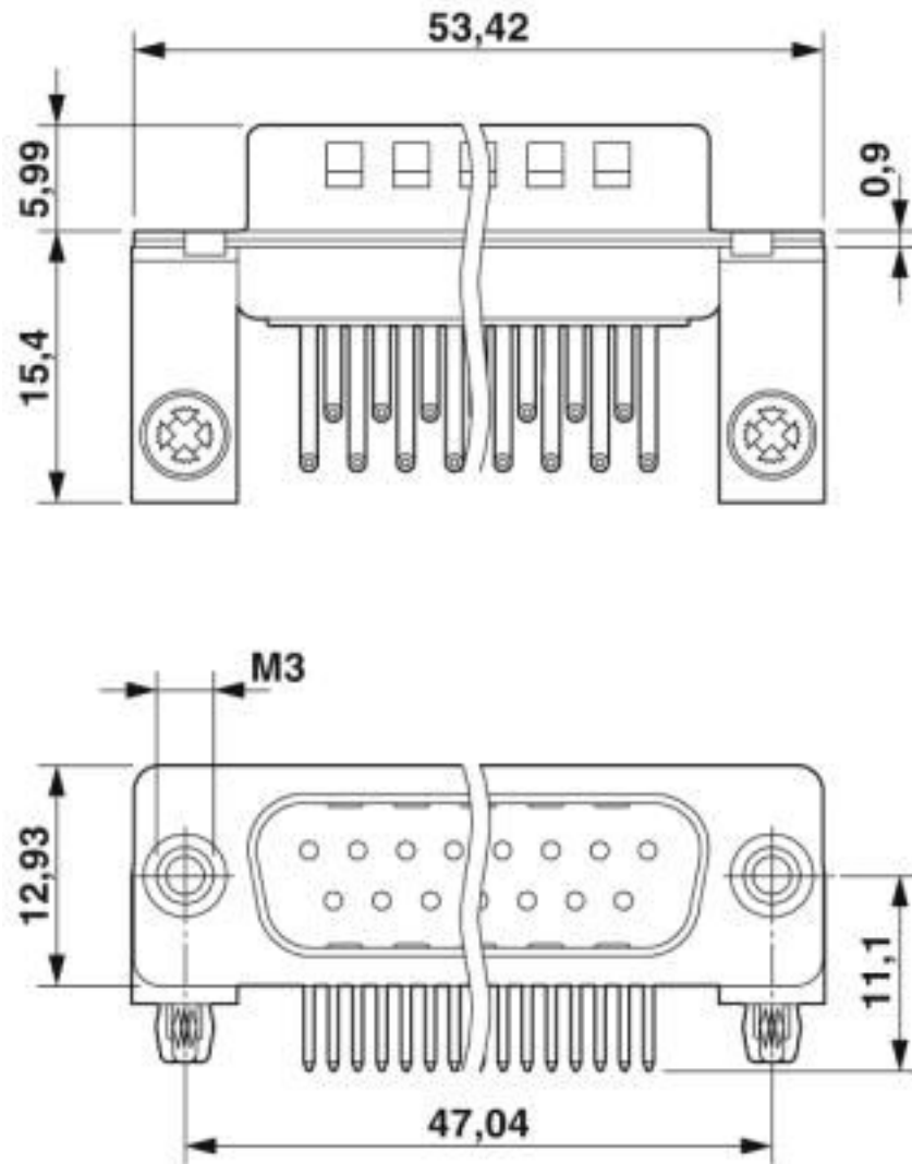
Dimensional drawing
