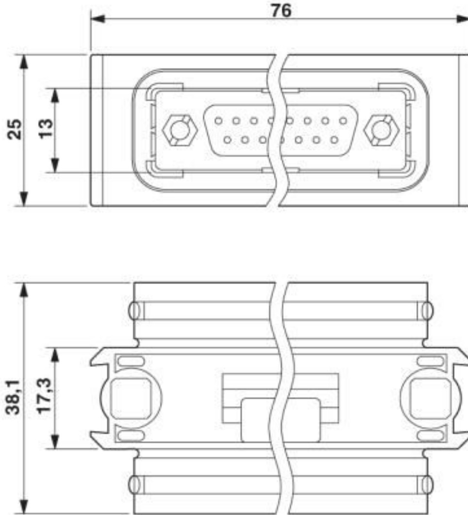
Dimensional drawing
