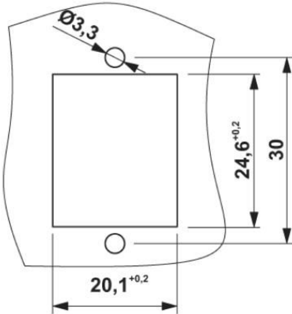
Dimensional drawing
