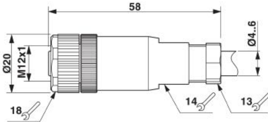
Dimensional drawing
