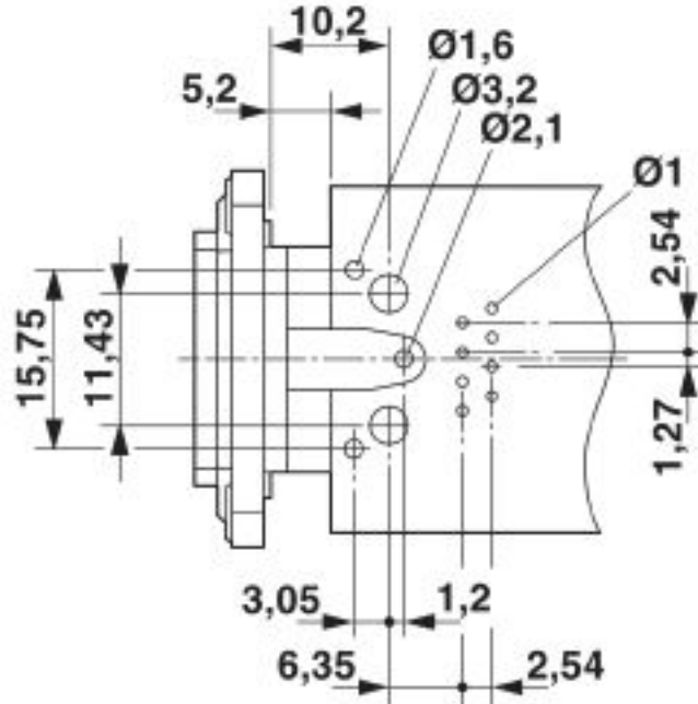
Drilling diagram
