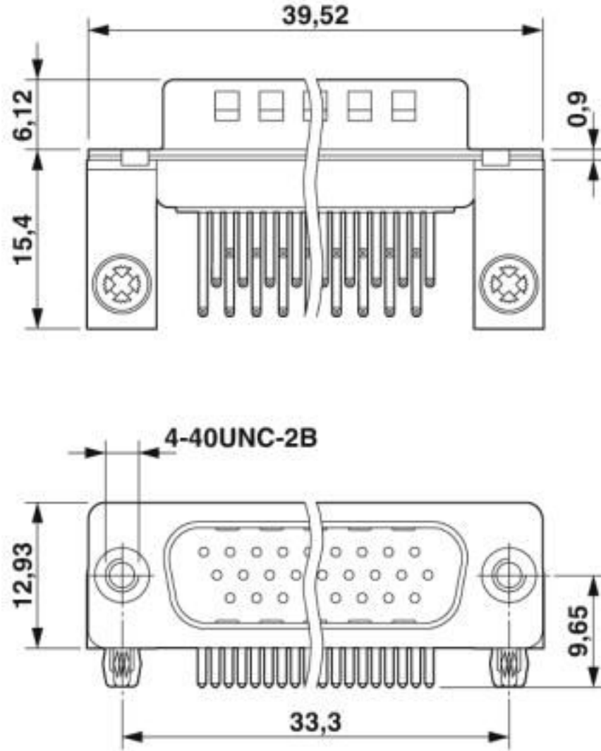
Dimensional drawing
