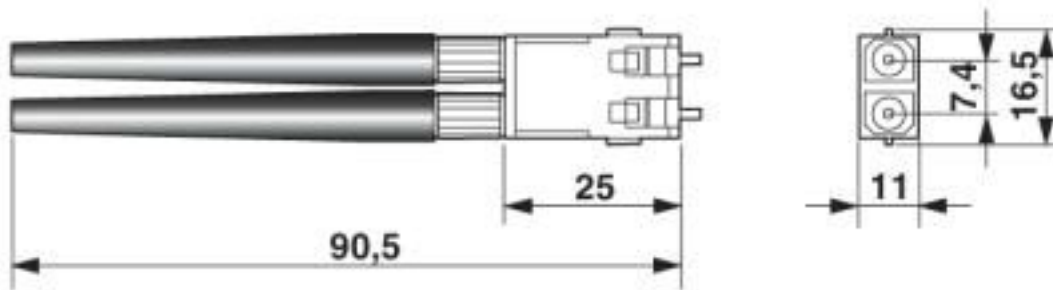
Dimensional drawing
