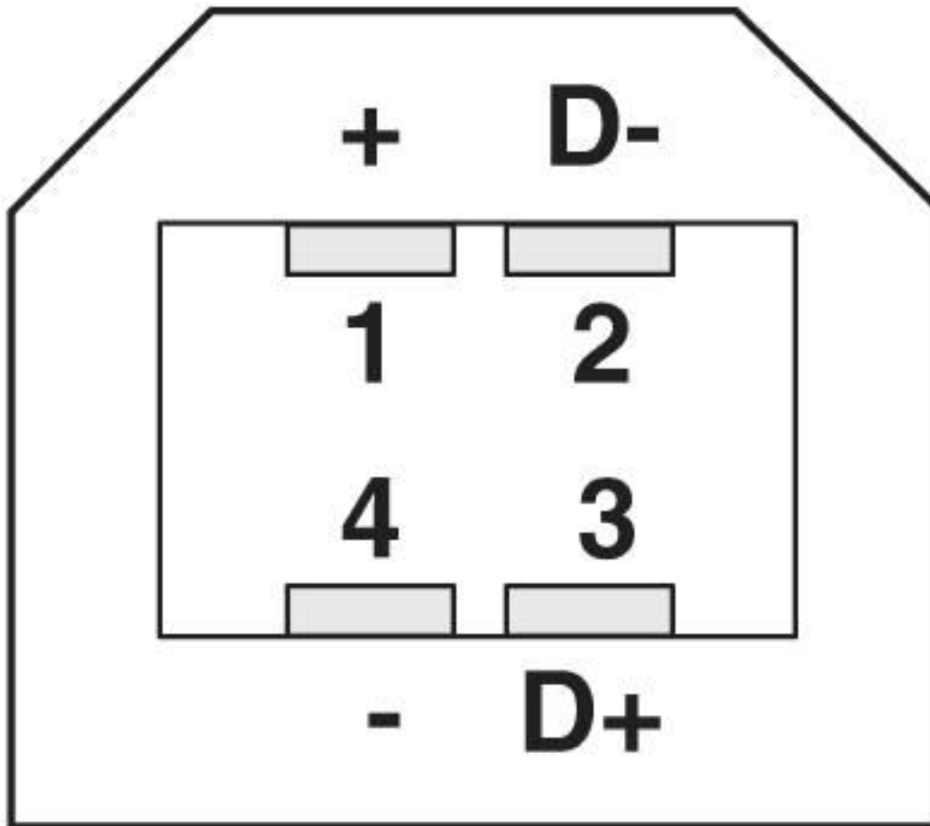
Pin assignment socket USB, type B
