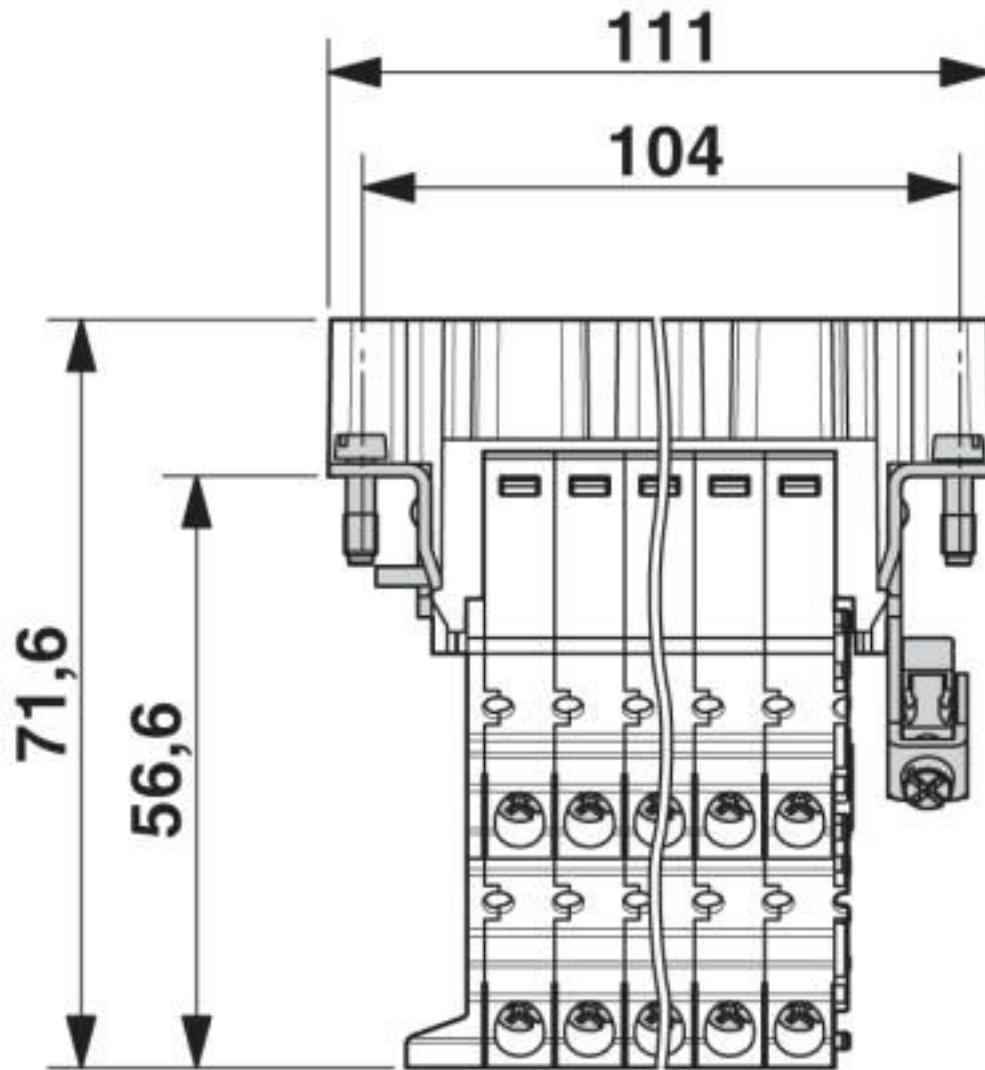
Dimensional drawing
