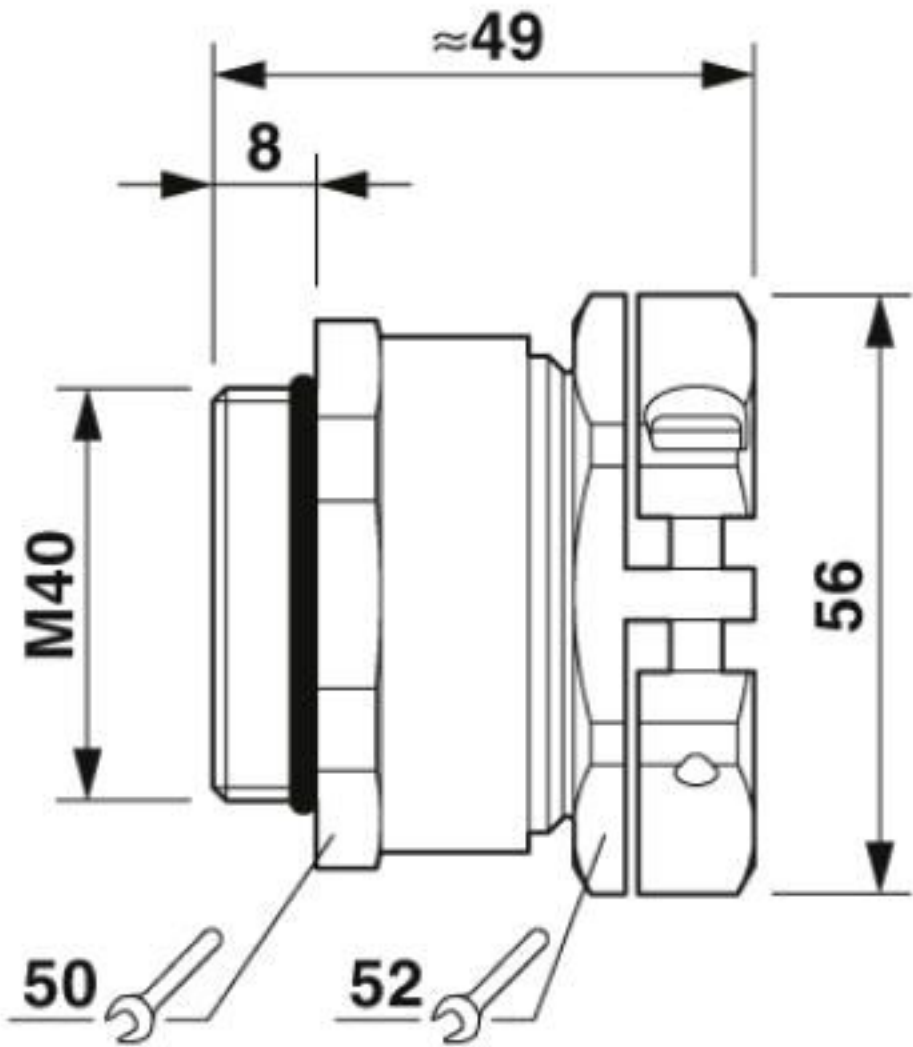
Dimensional drawing
