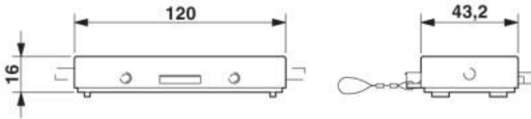
Dimensional drawing
