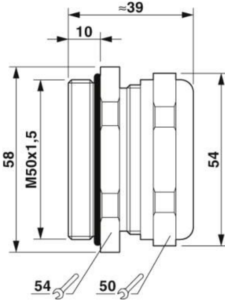
Dimensional drawing
