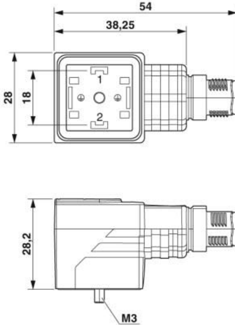
Dimensional drawing
