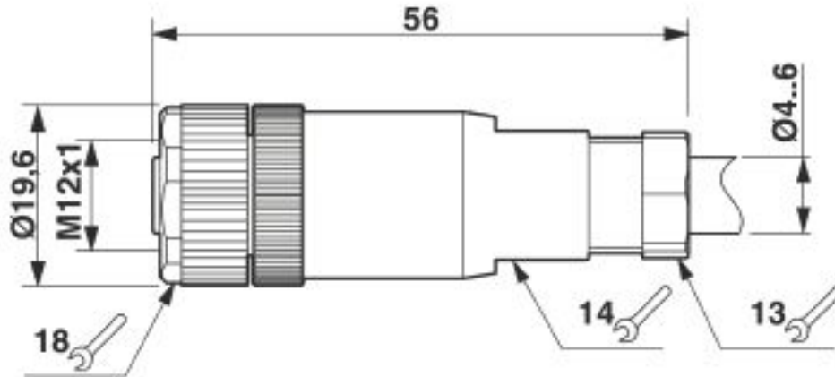
Dimensional drawing
